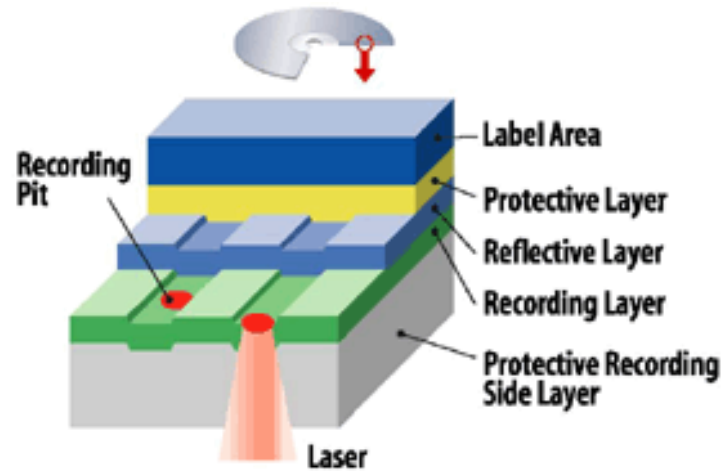
CD-R Structural Cross Section
